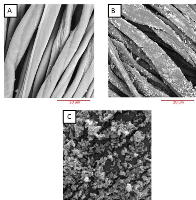
Figure 1. SEM images (A untreated, B ZnO NPs deposited sample, C ZnO NPs deposited sample at high resolution)
