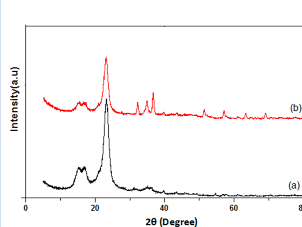
Figure 2. XRD patterns (a) untreated fabric (b) ZnO coated fabric
